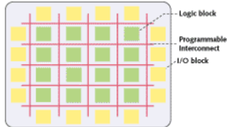
Figure 2. Internal structure of an FPGA
